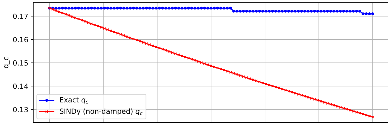
Trajectory 2139 (non-damped)
