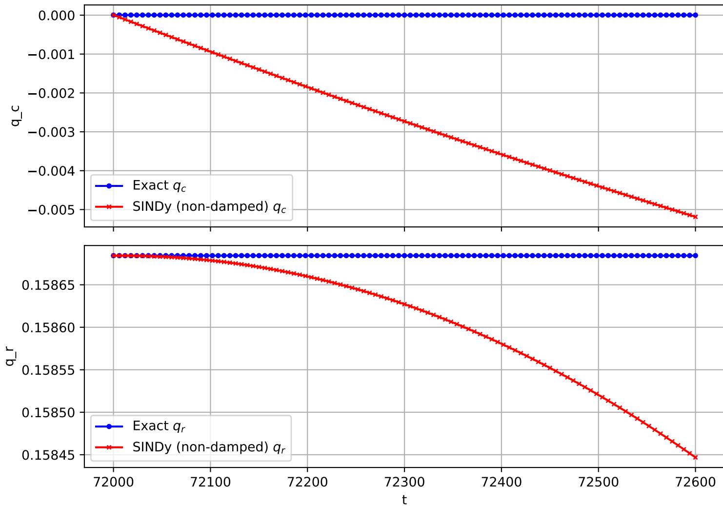
Trajectory 2141 (non-damped)
