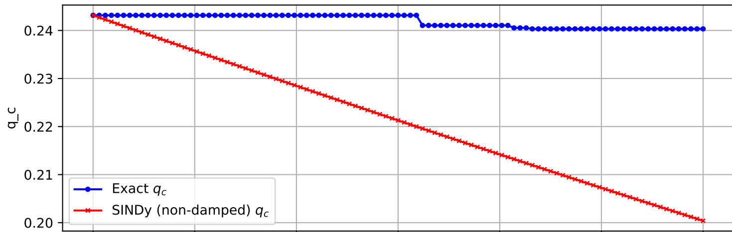
Trajectory 2146 (non-damped)
