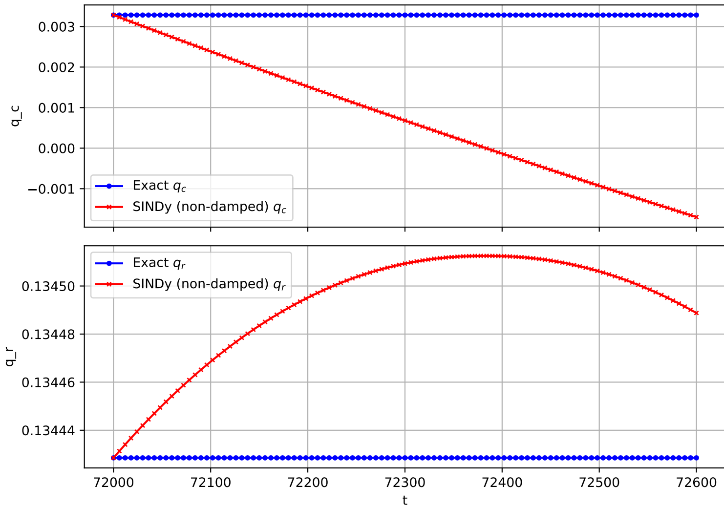
Trajectory 2153 (non-damped)
