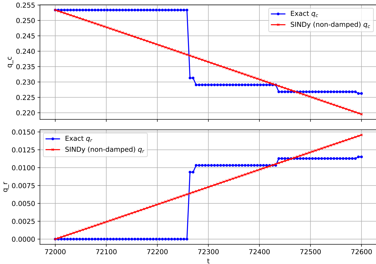
Trajectory 2156 (non-damped)
