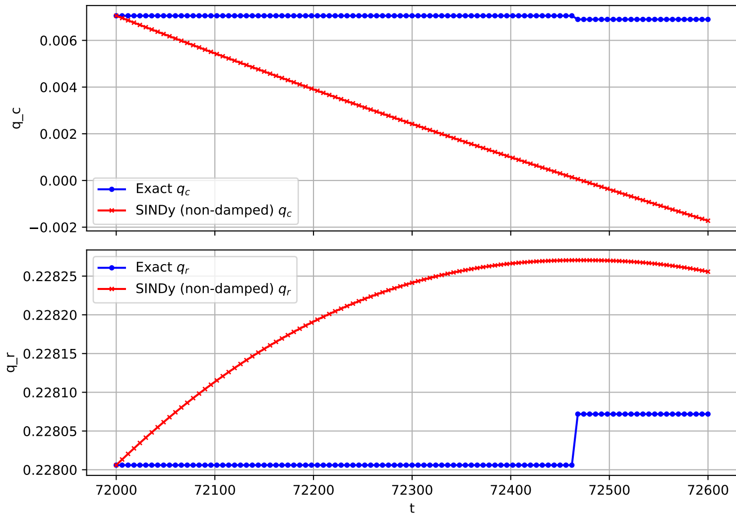
Trajectory 2158 (non-damped)
