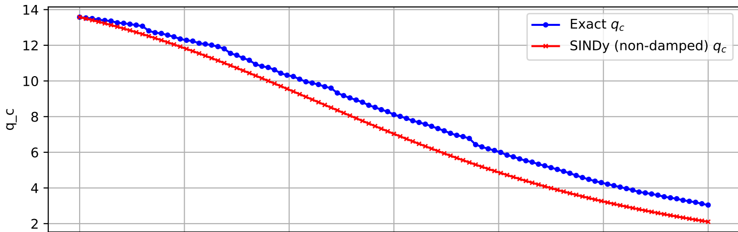
Trajectory 2164 (non-damped)
