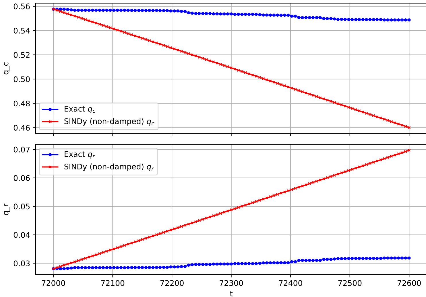
Trajectory 2168 (non-damped)
