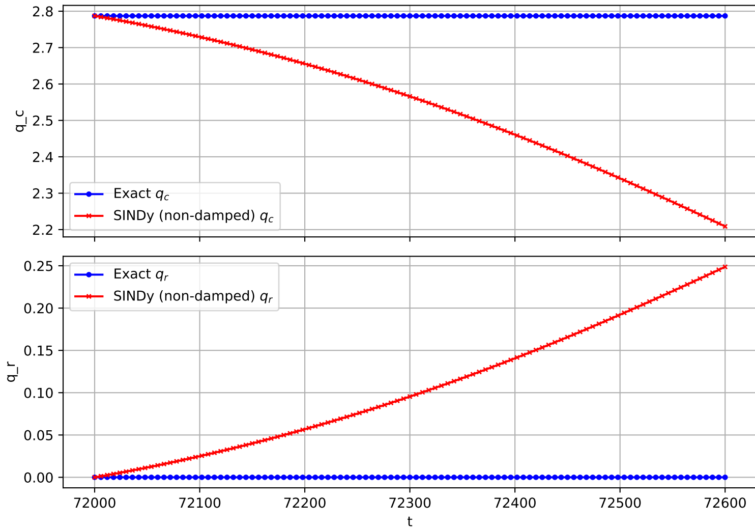
Trajectory 2181 (non-damped)
