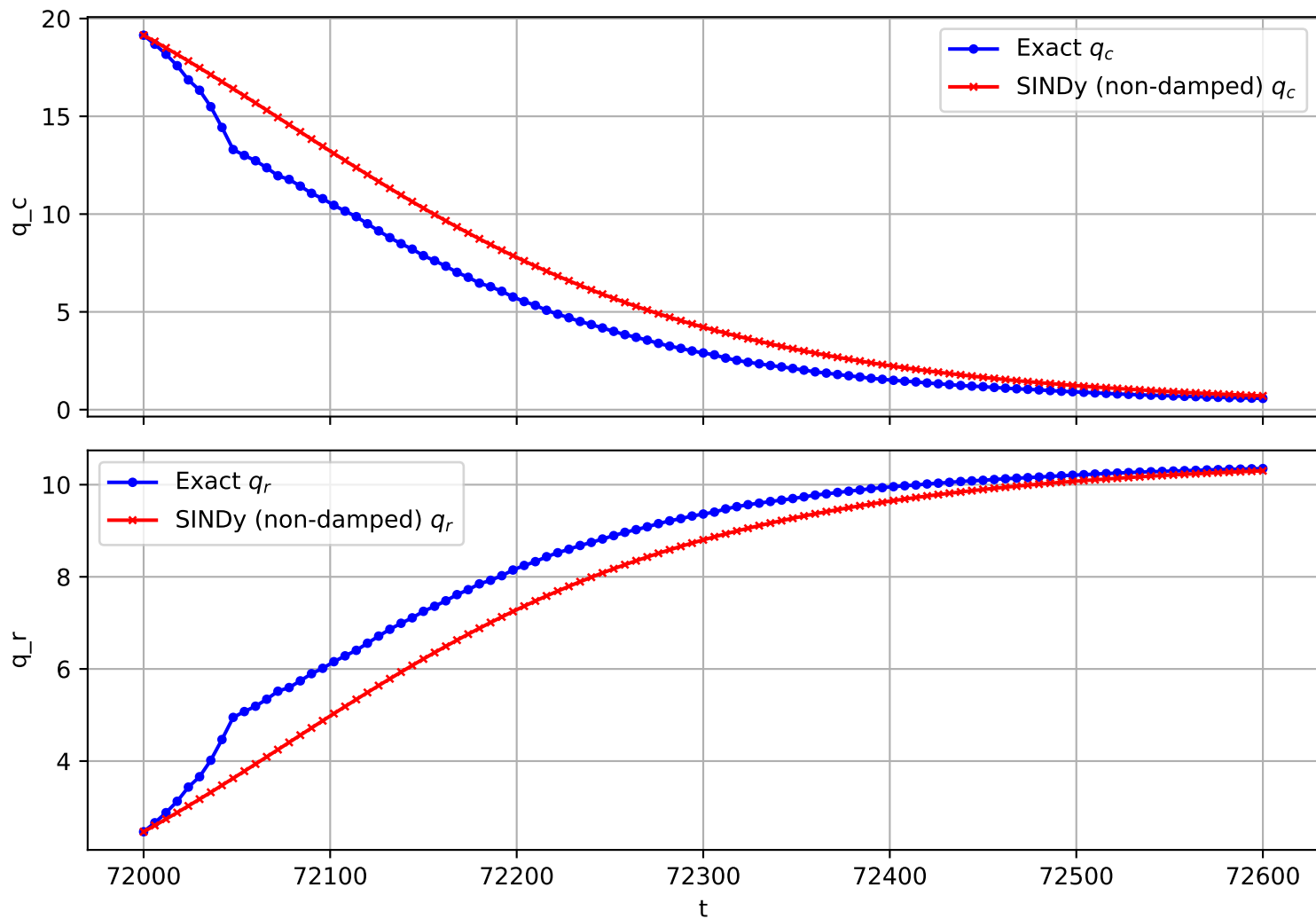
Trajectory 2183 (non-damped)
