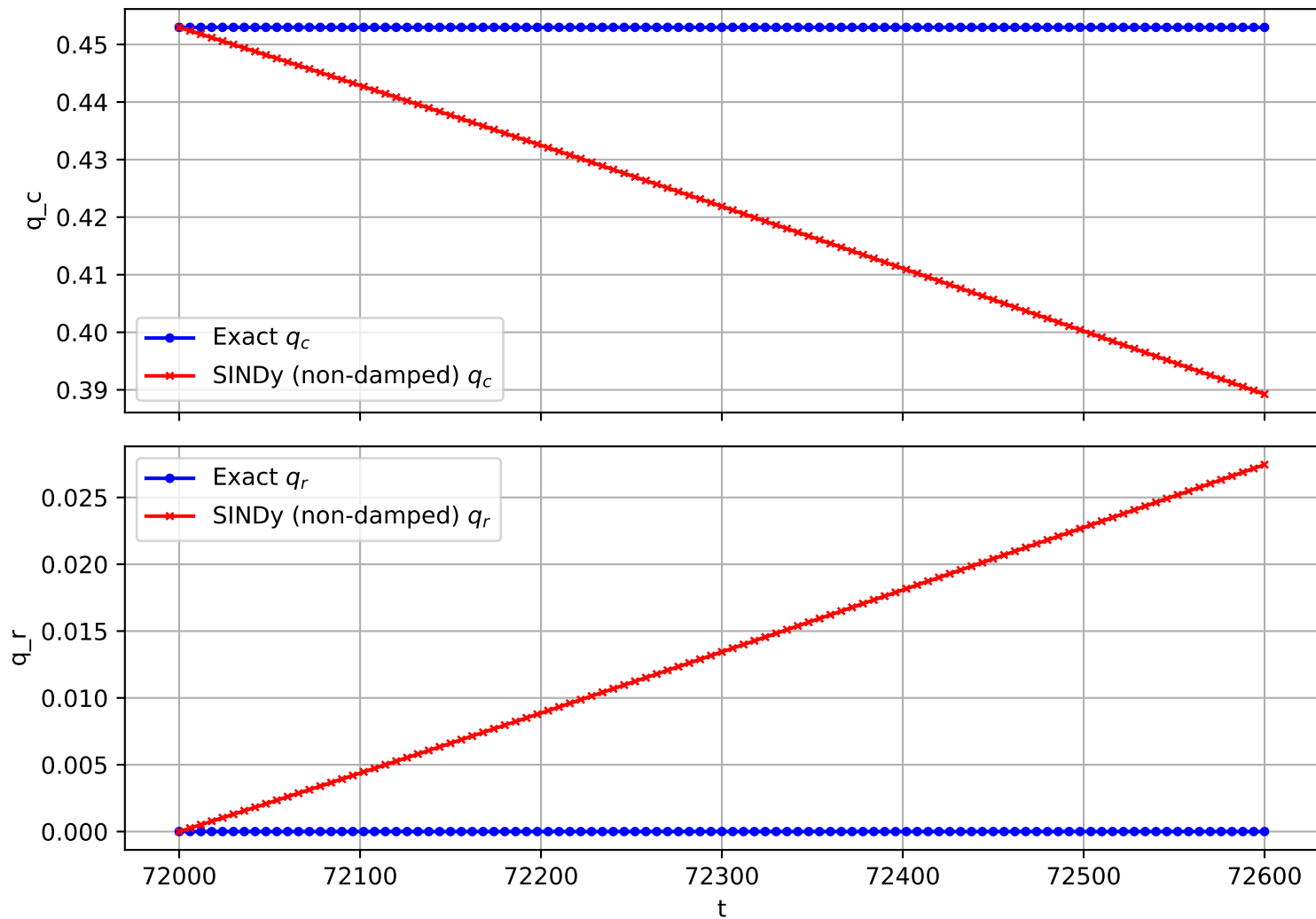
Trajectory 2196 (non-damped)
