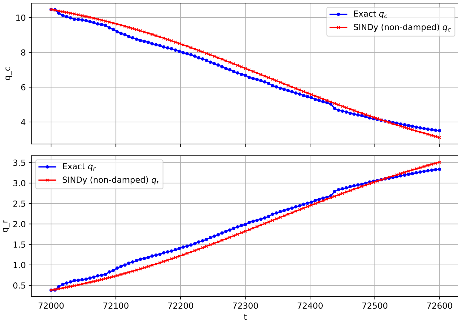
Trajectory 2205 (non-damped)
