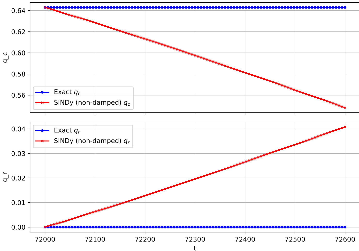
Trajectory 2208 (non-damped)
