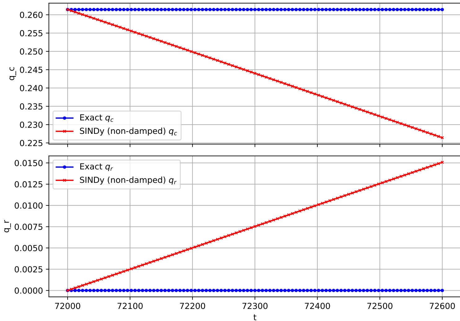
Trajectory 2211 (non-damped)
