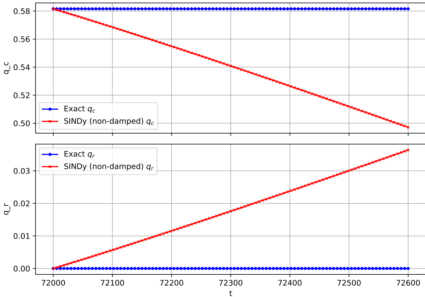
Trajectory 2216 (non-damped)
