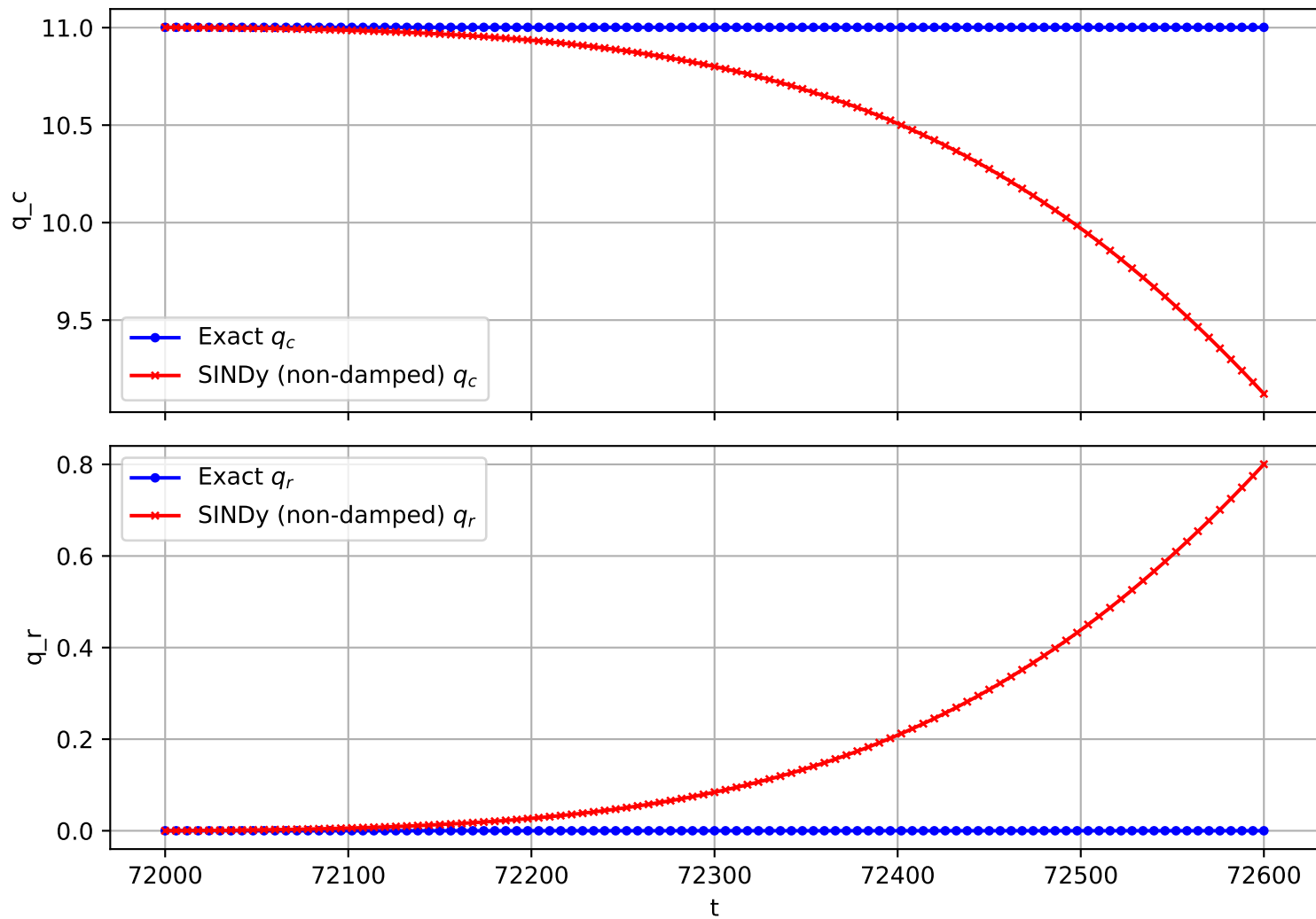
Trajectory 2218 (non-damped)
