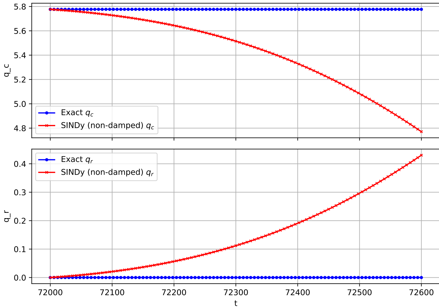
Trajectory 2224 (non-damped)
