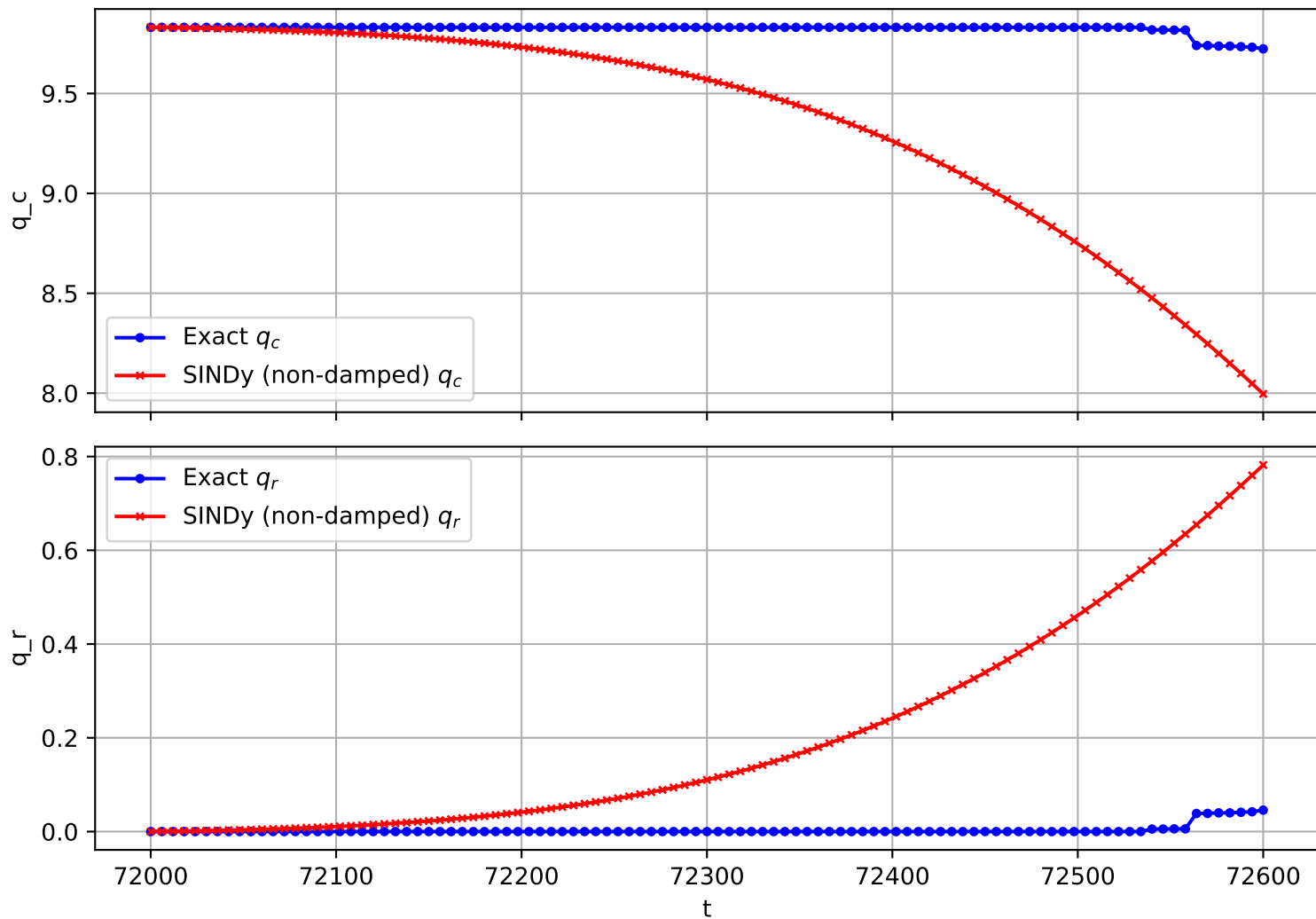
Trajectory 2226 (non-damped)
