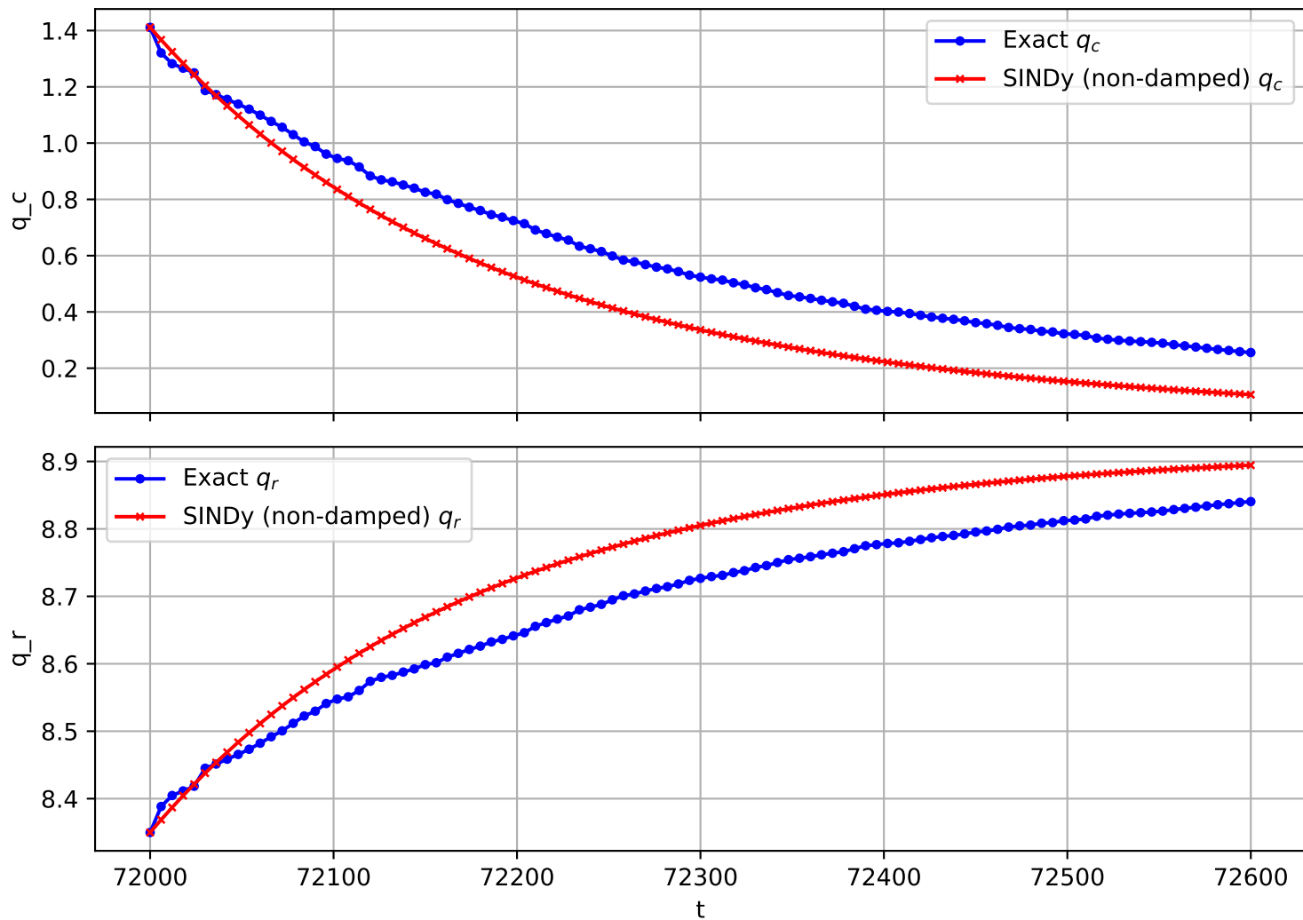
Trajectory 223 (non-damped)
