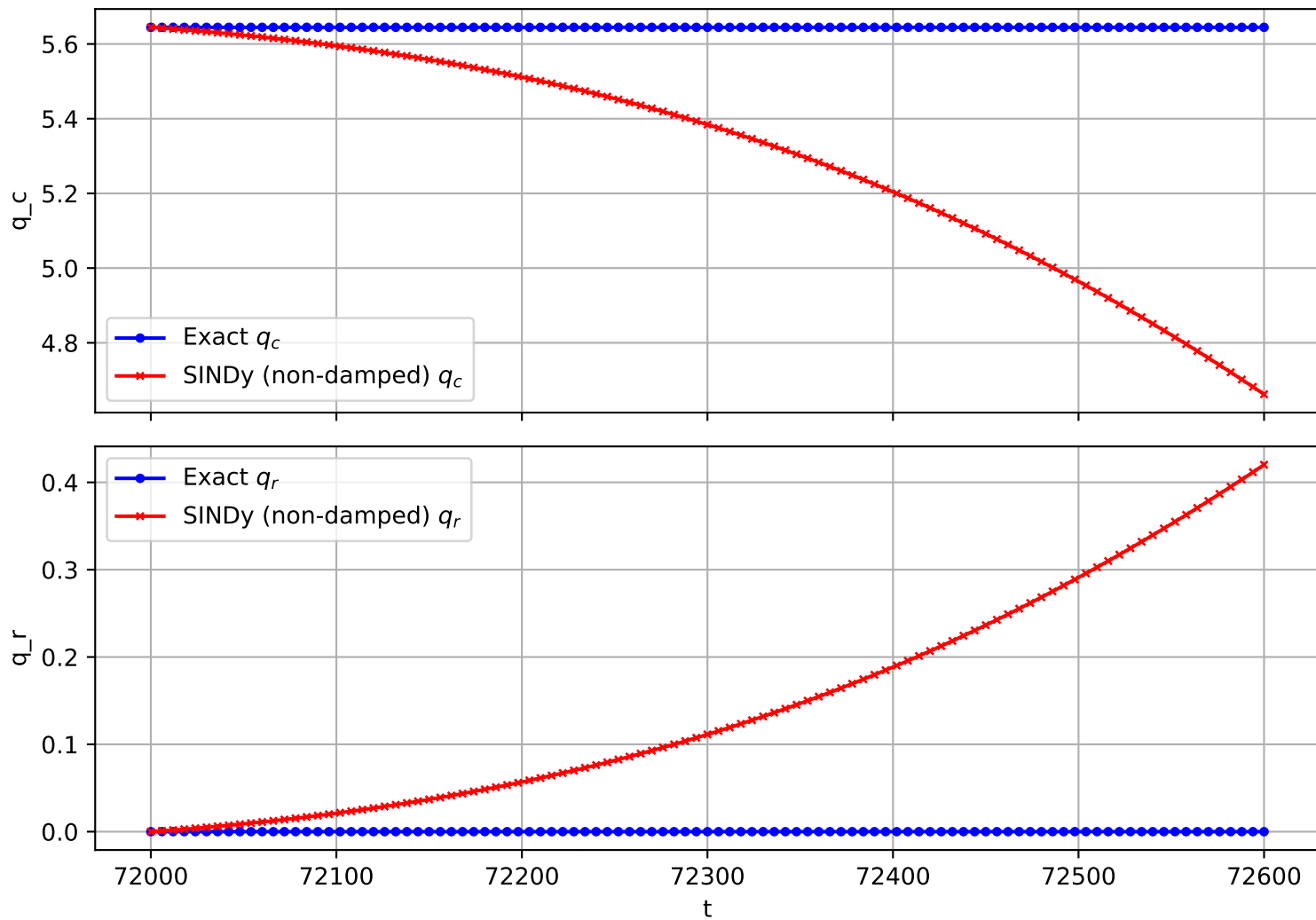
Trajectory 2240 (non-damped)
