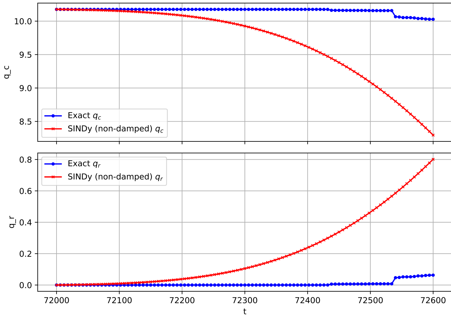
Trajectory 2244 (non-damped)
