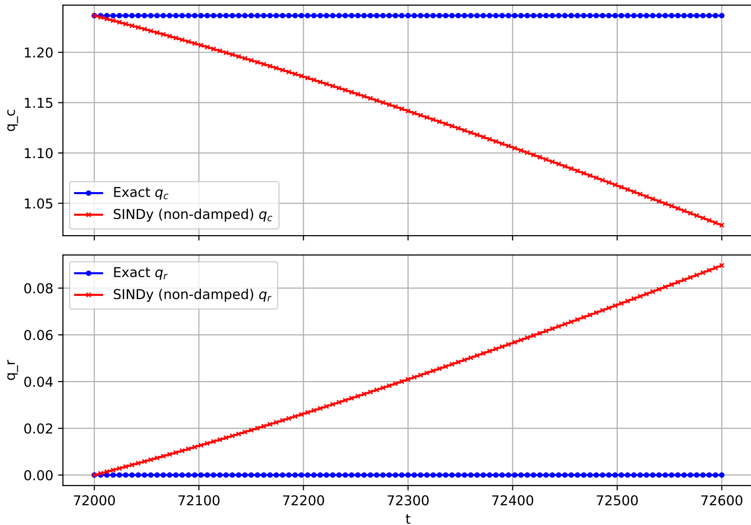
Trajectory 2246 (non-damped)
