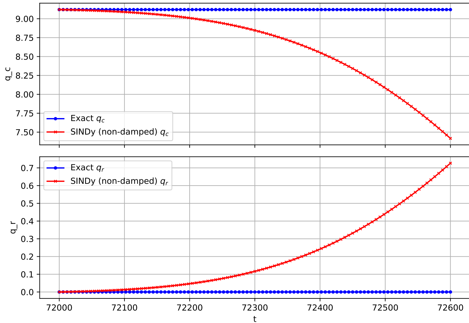
Trajectory 2249 (non-damped)
