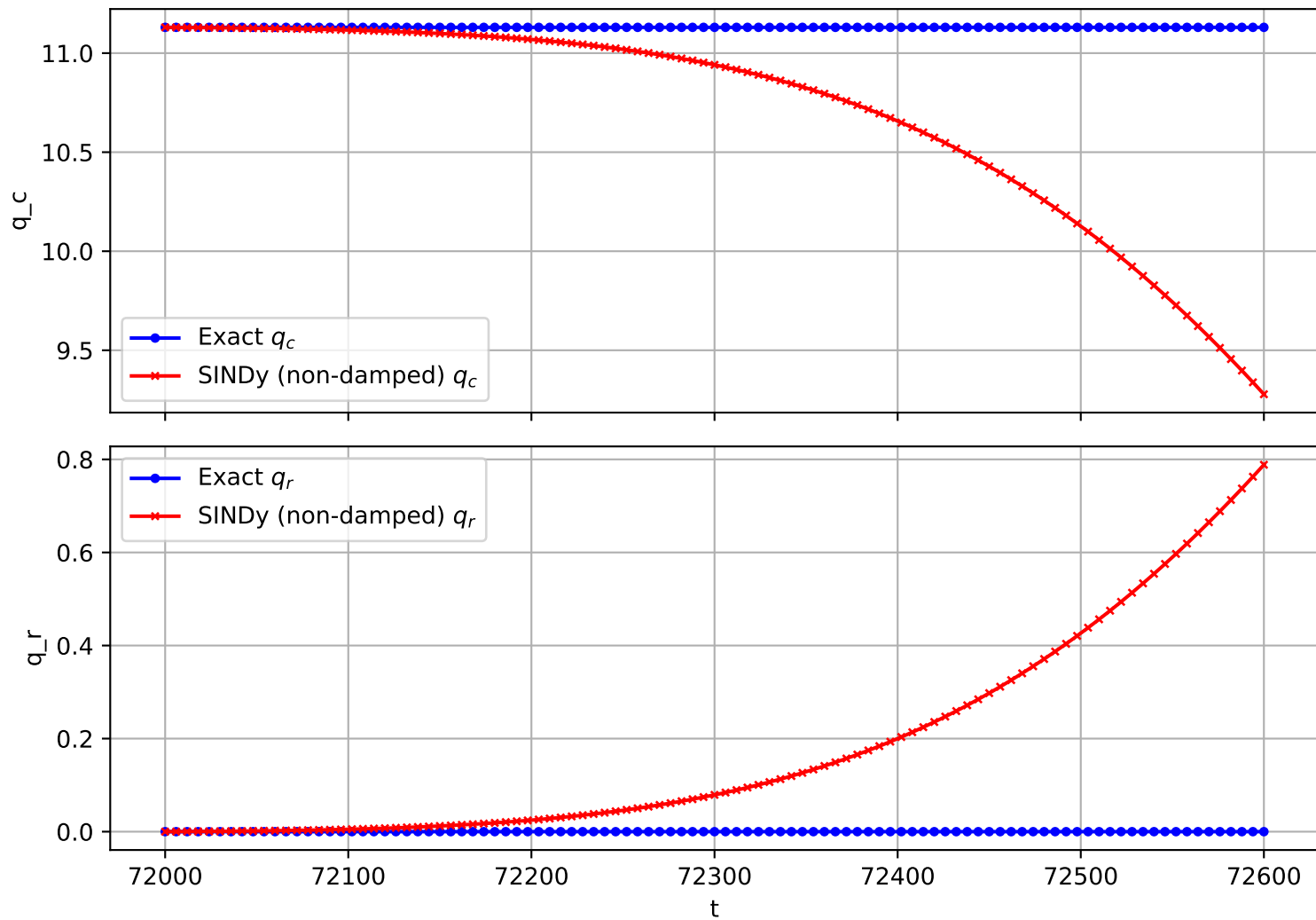
Trajectory 2250 (non-damped)
