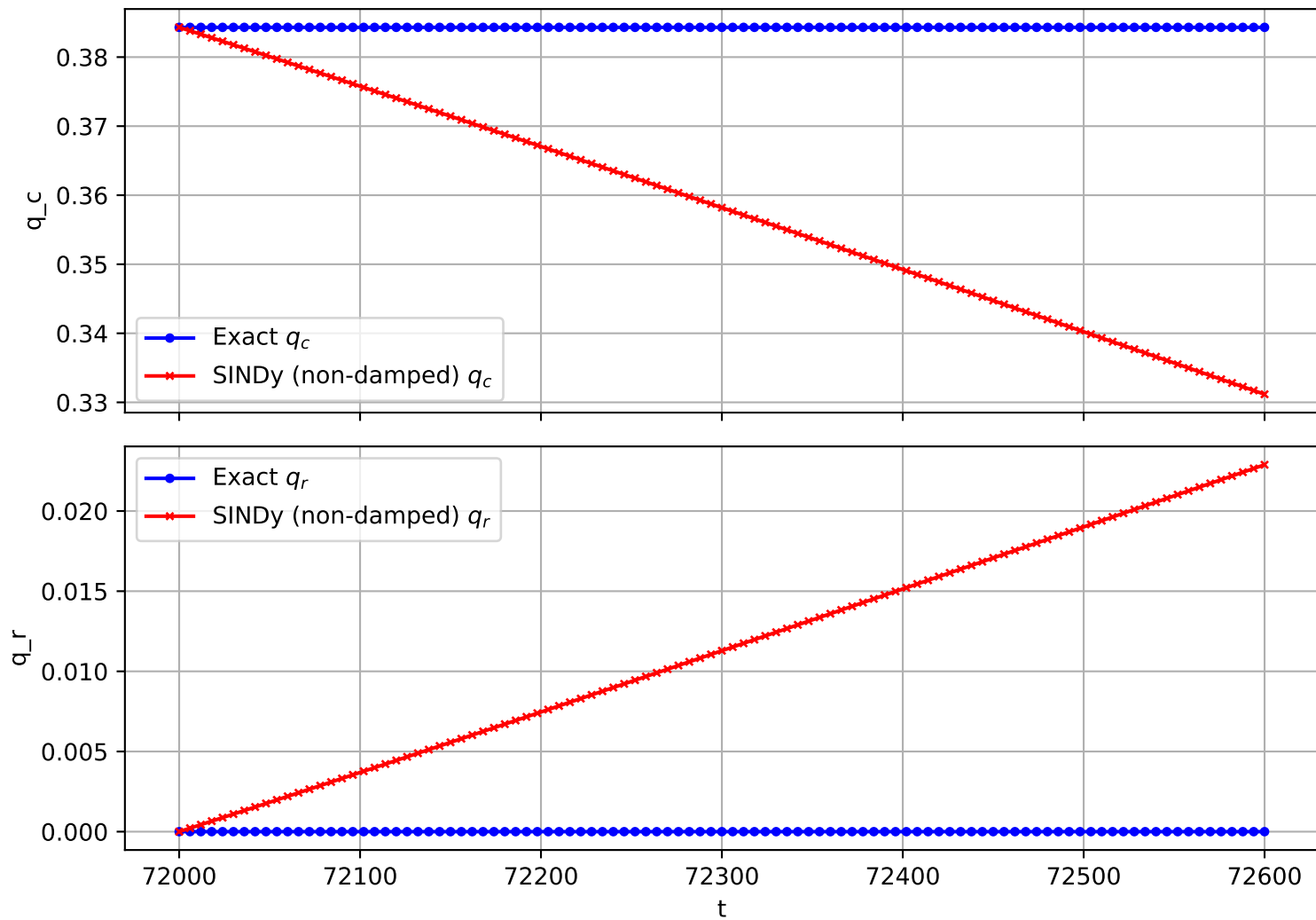
Trajectory 2265 (non-damped)
