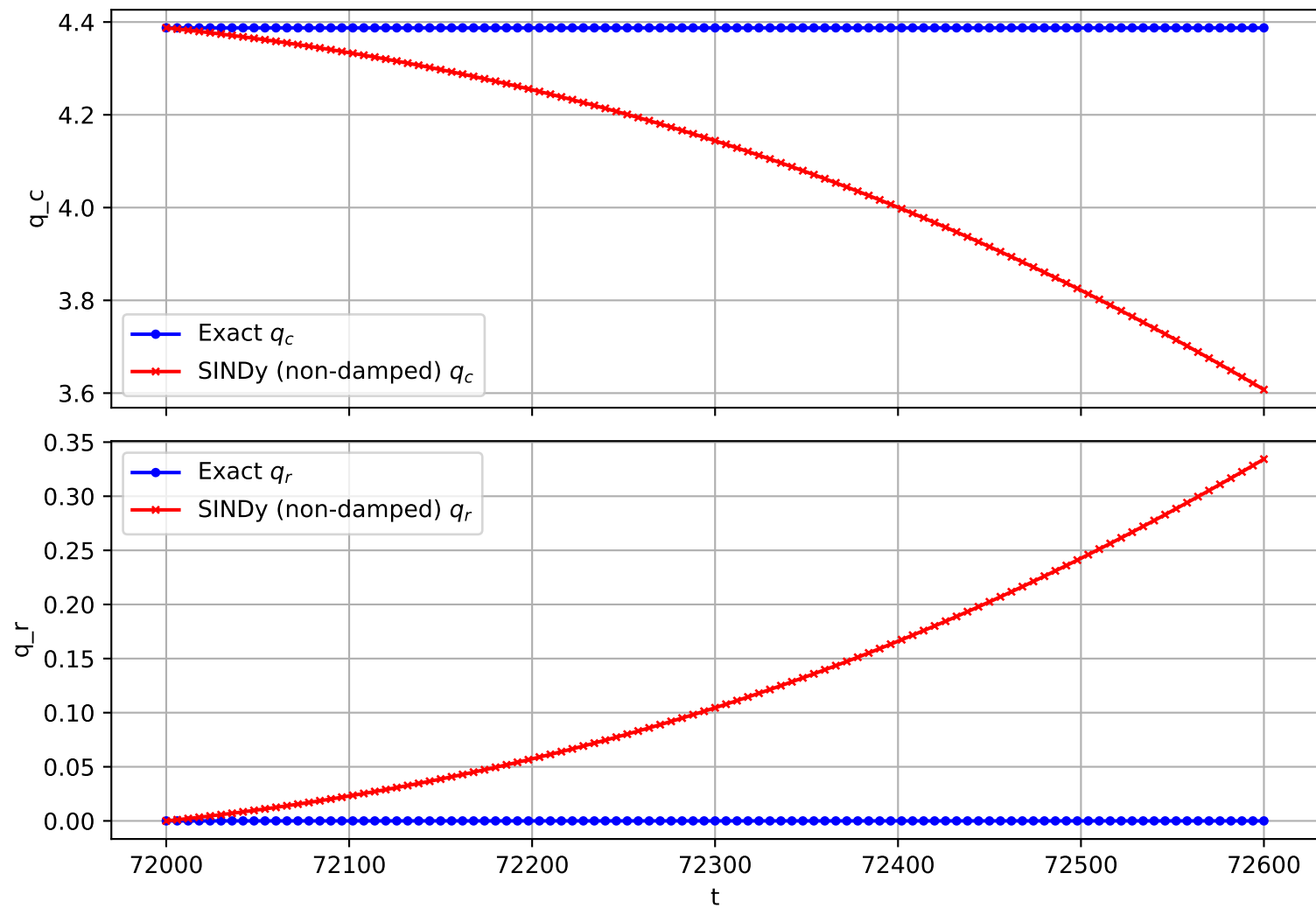
Trajectory 2275 (non-damped)
