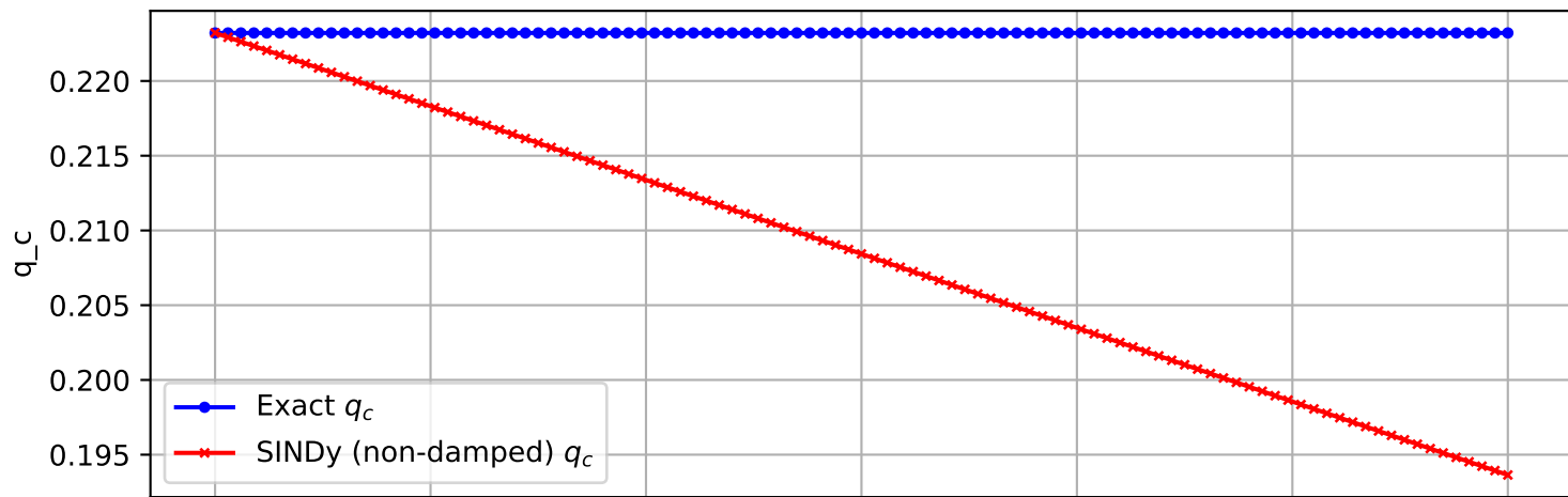
Trajectory 2286 (non-damped)
