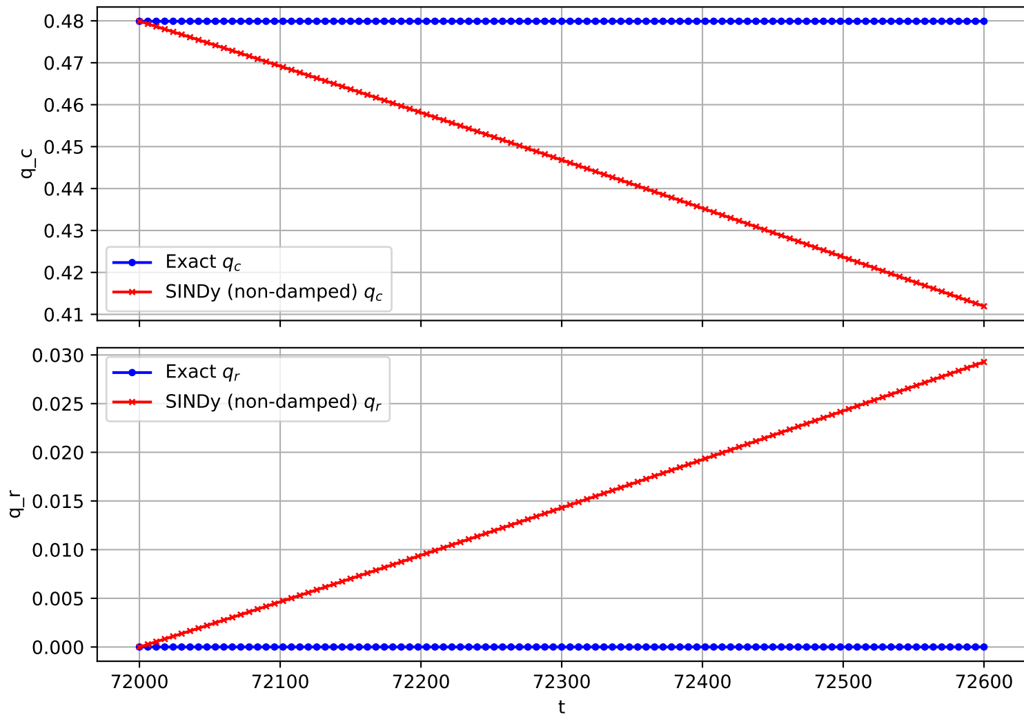
Trajectory 2288 (non-damped)
