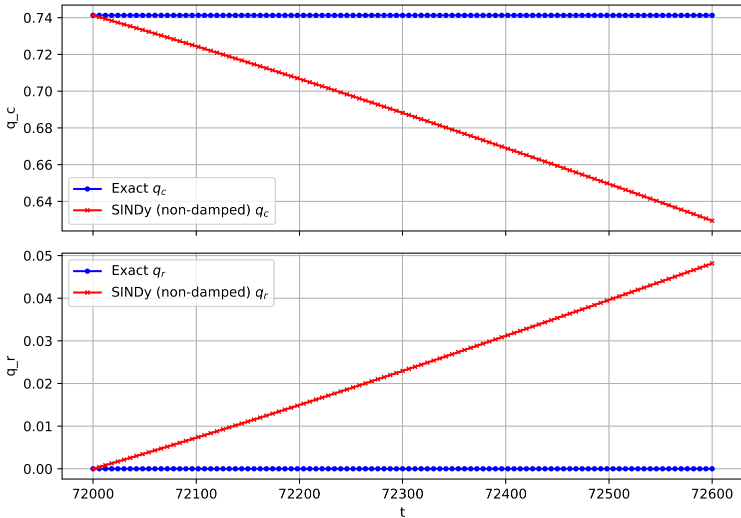
Trajectory 2291 (non-damped)
