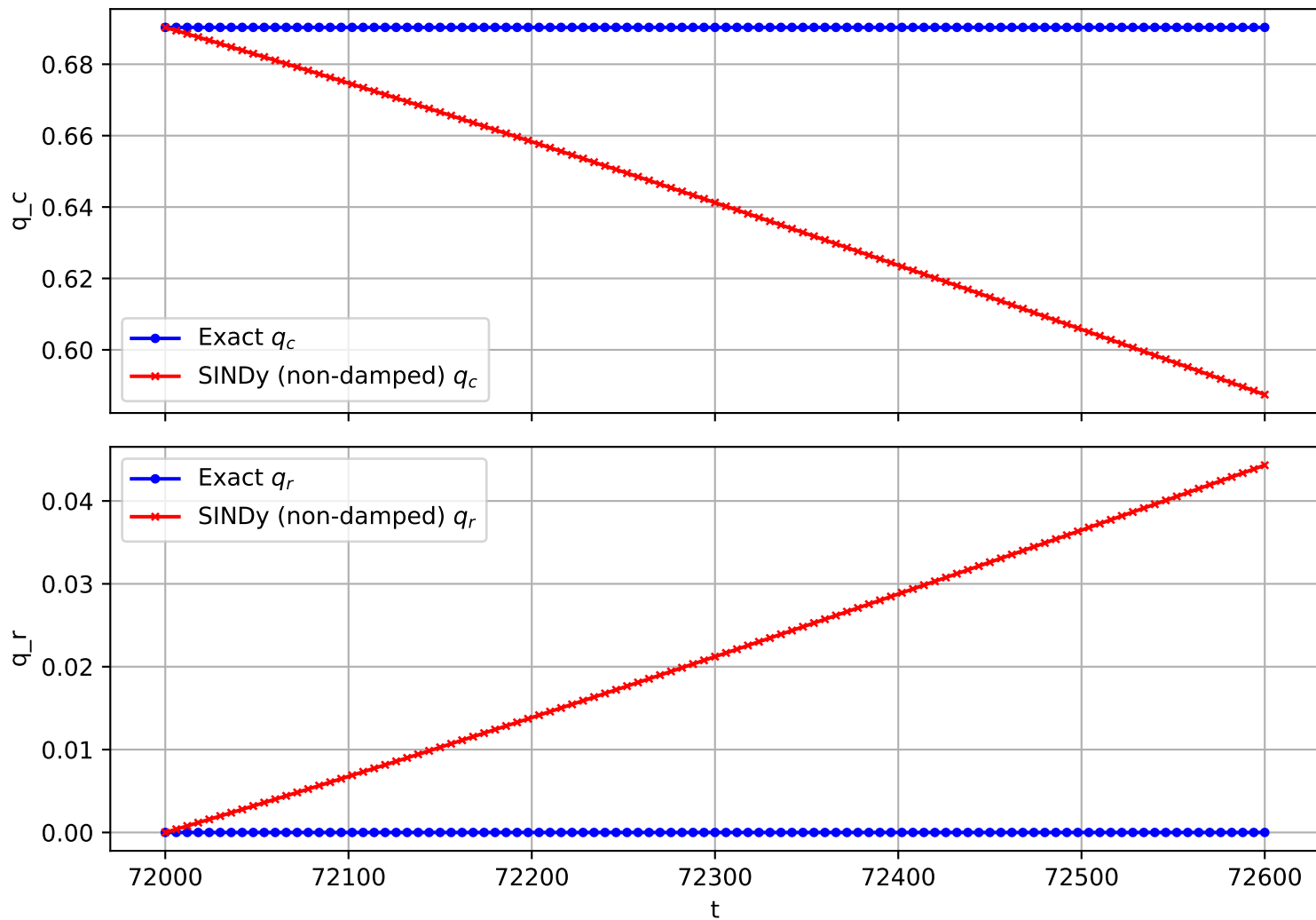
Trajectory 2295 (non-damped)
