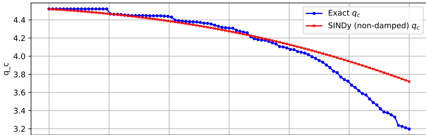
Trajectory 2299 (non-damped)
