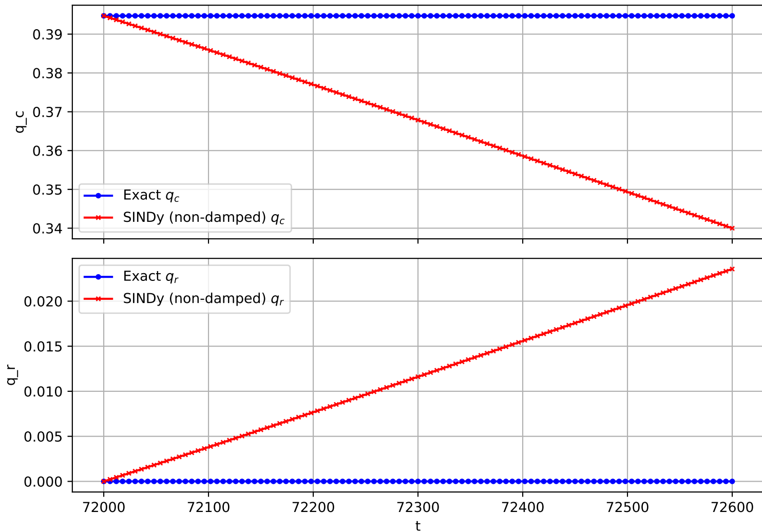
Trajectory 2300 (non-damped)
