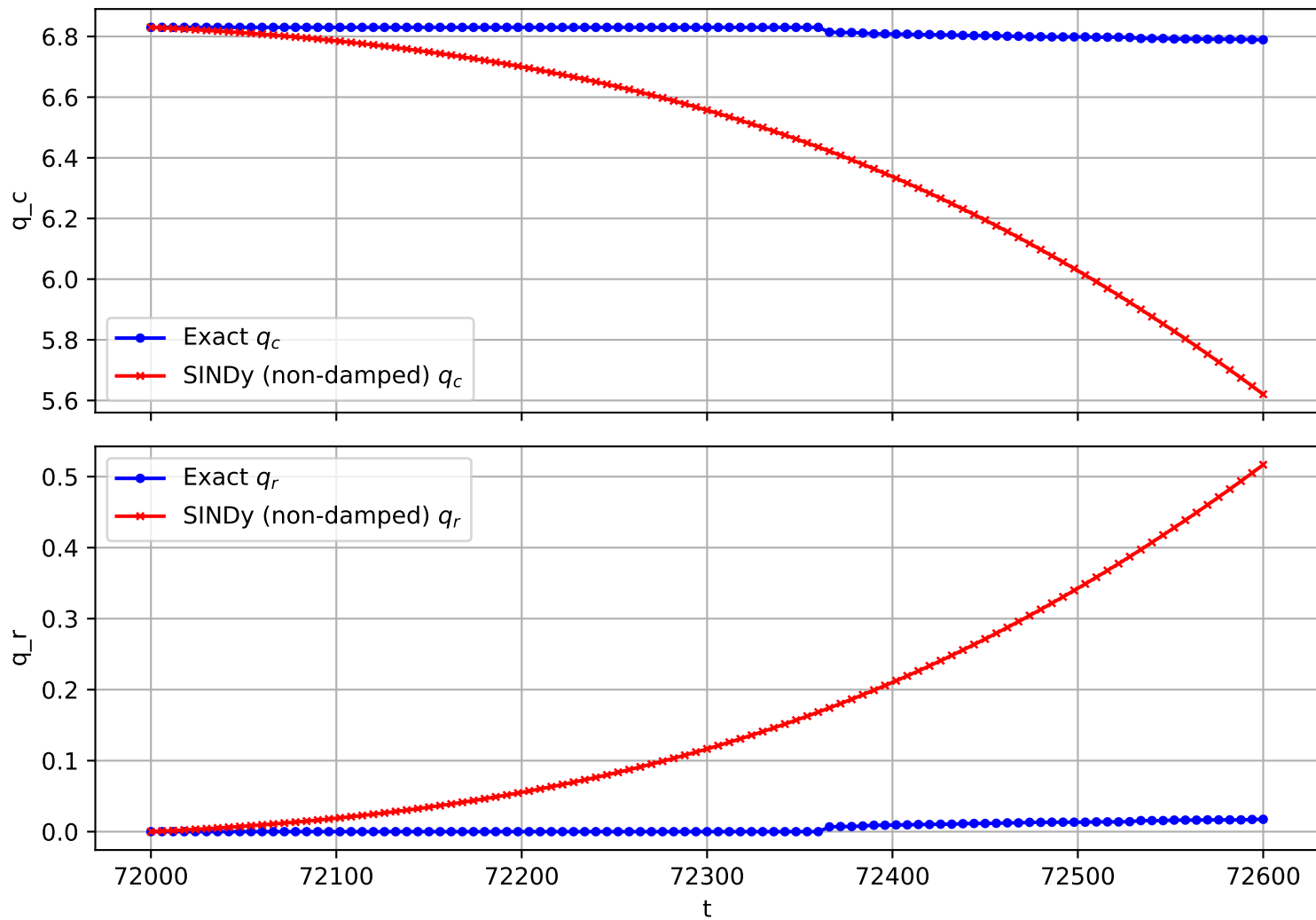
Trajectory 2302 (non-damped)
