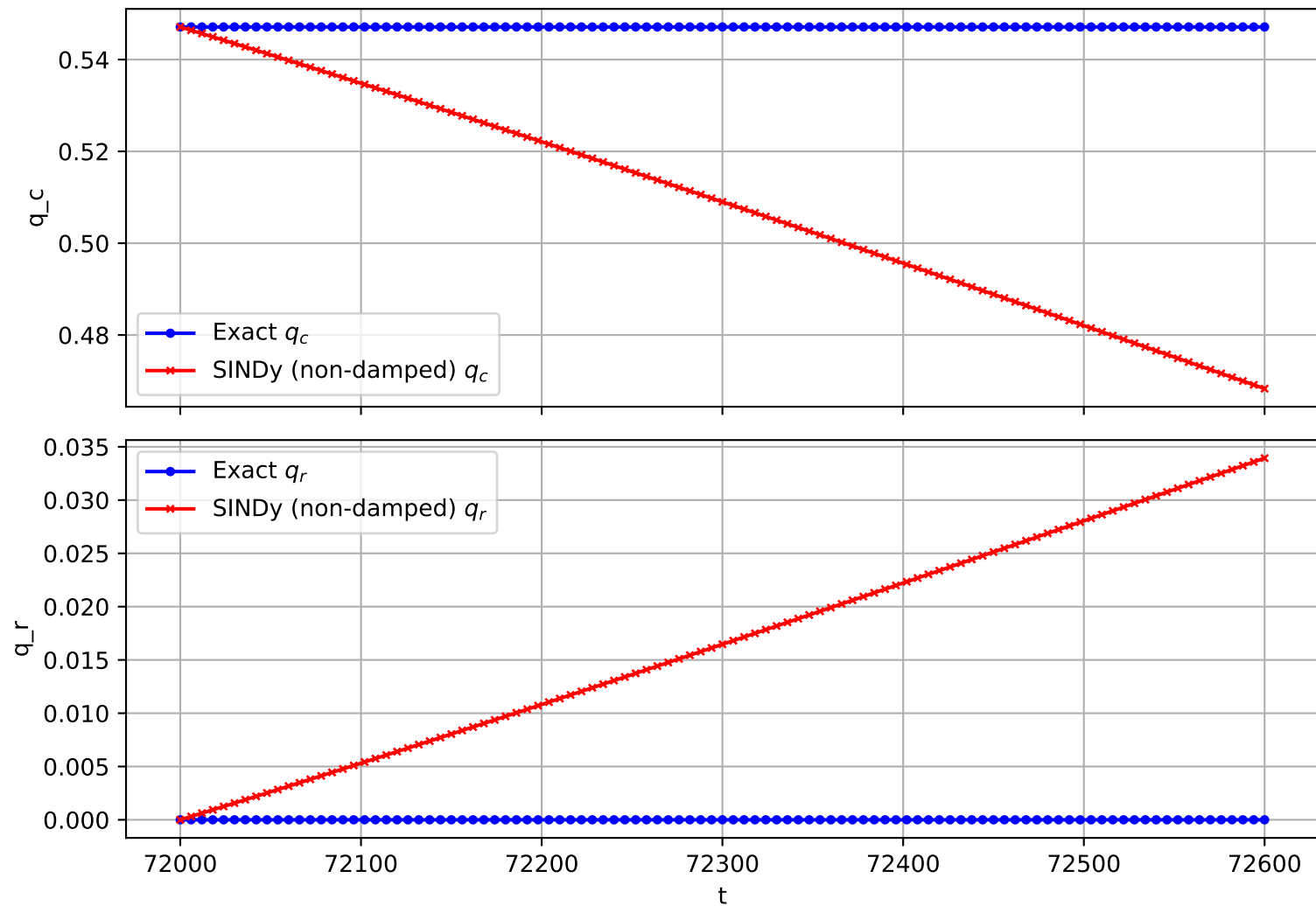
Trajectory 2304 (non-damped)
