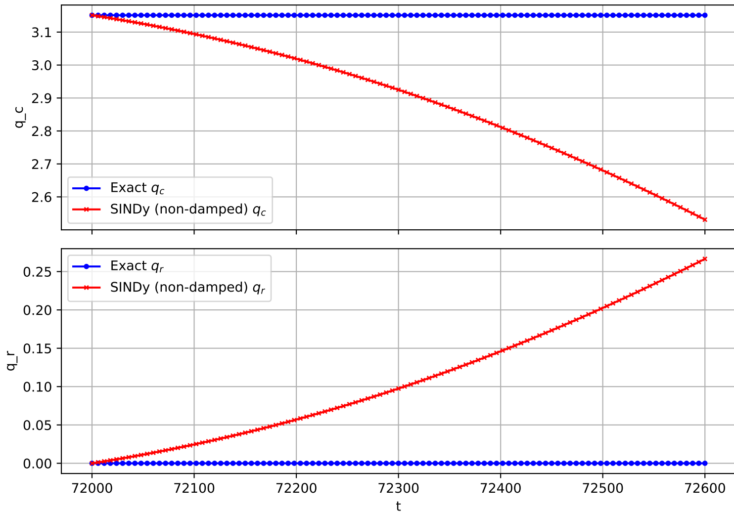
Trajectory 2333 (non-damped)
