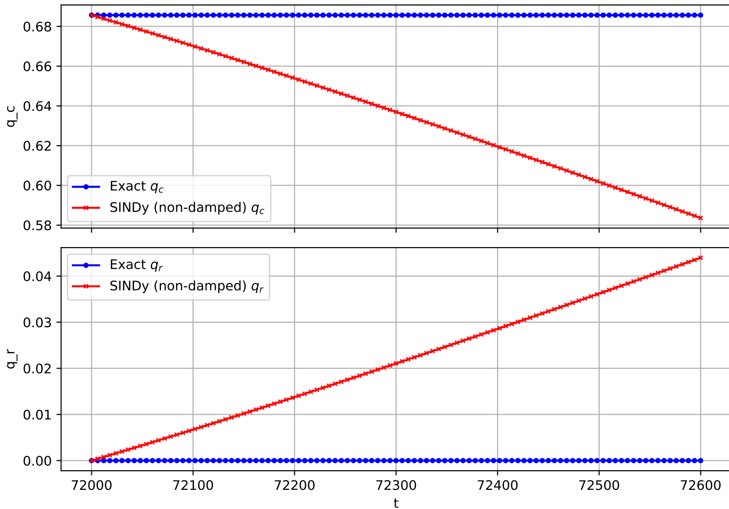
Trajectory 2336 (non-damped)
