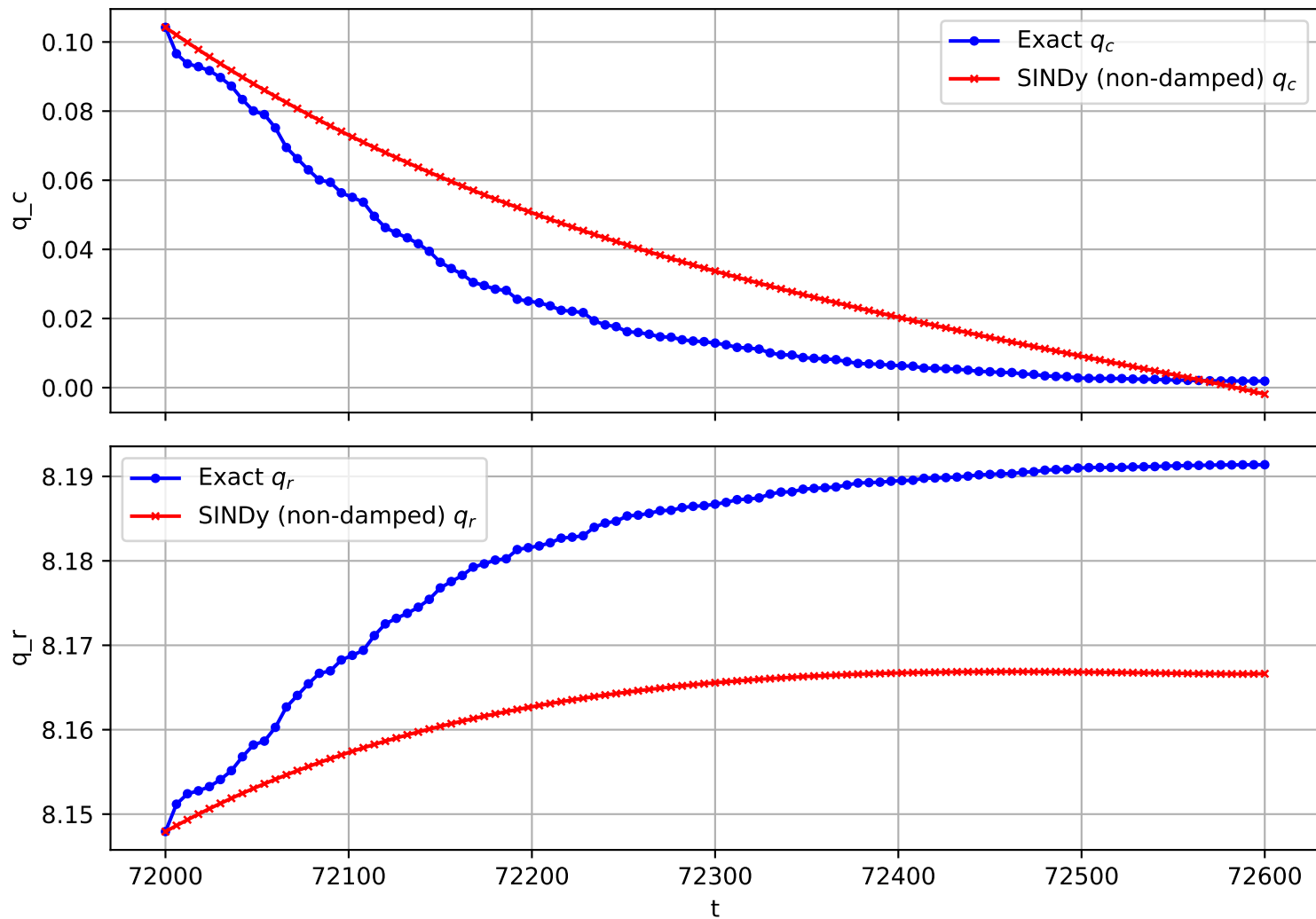
Trajectory 234 (non-damped)
