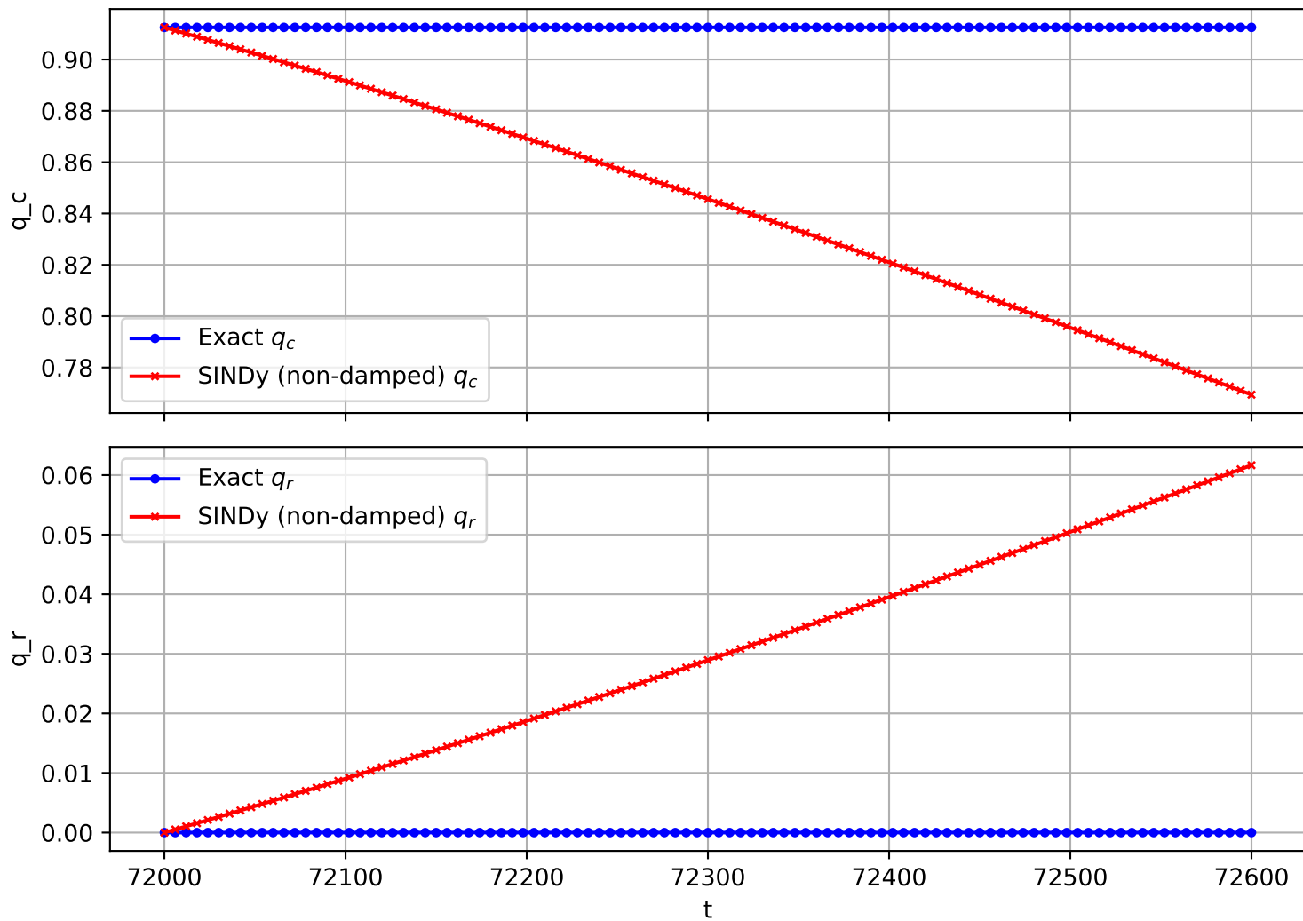
Trajectory 2340 (non-damped)
