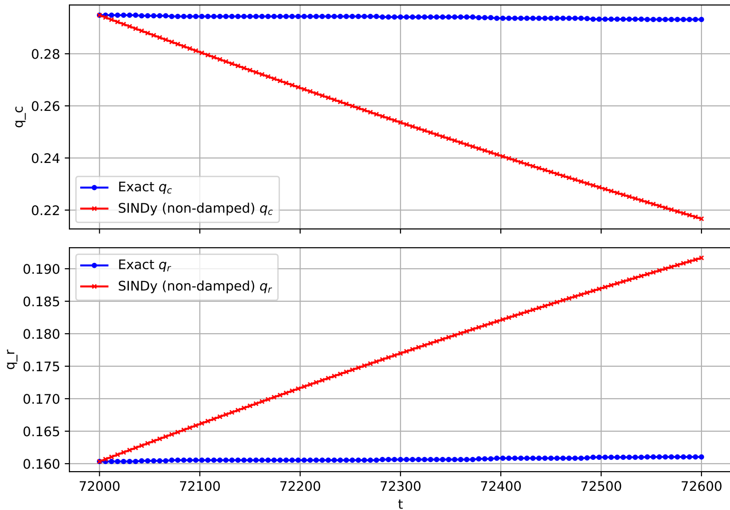
Trajectory 2349 (non-damped)
