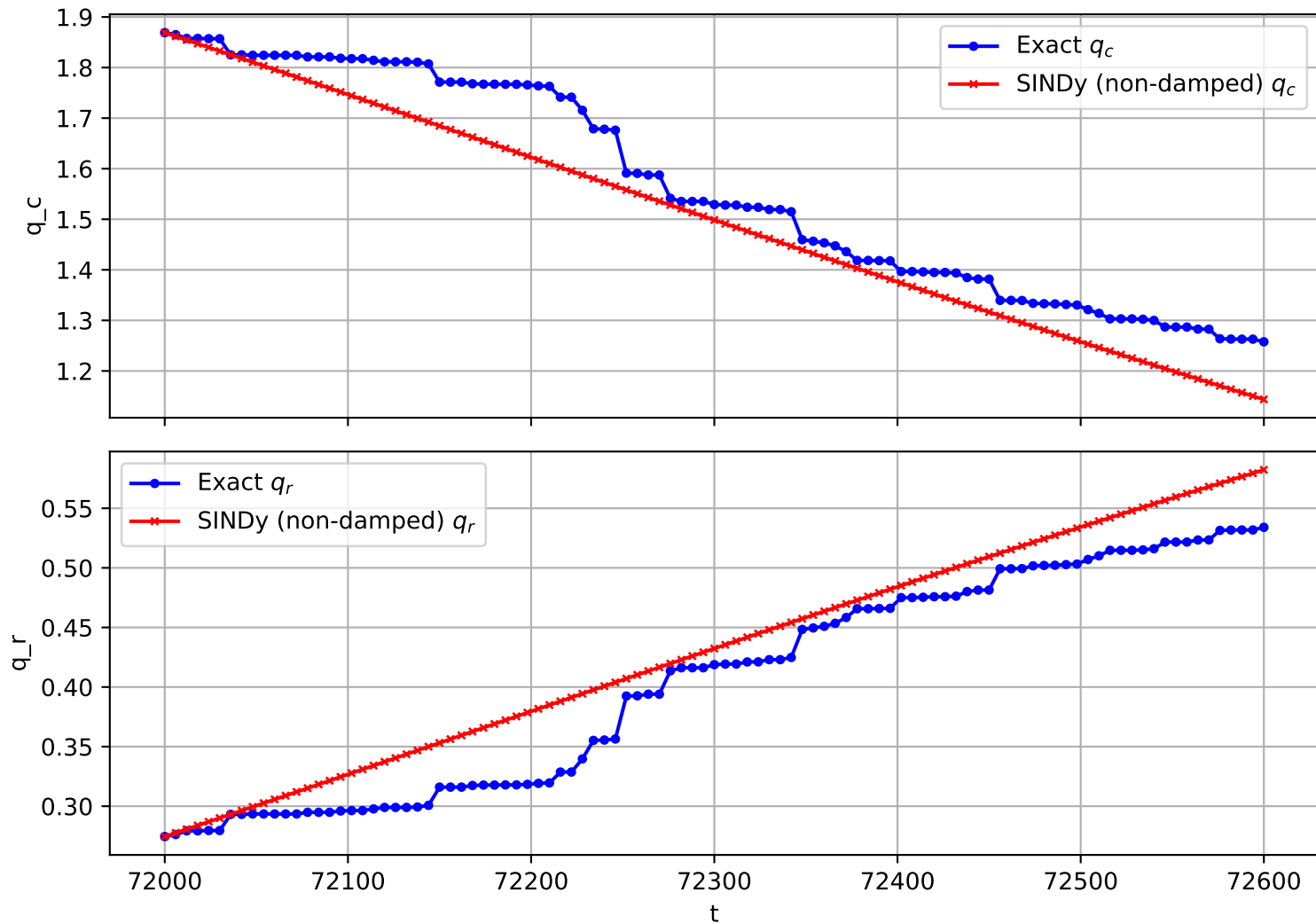
Trajectory 2350 (non-damped)
