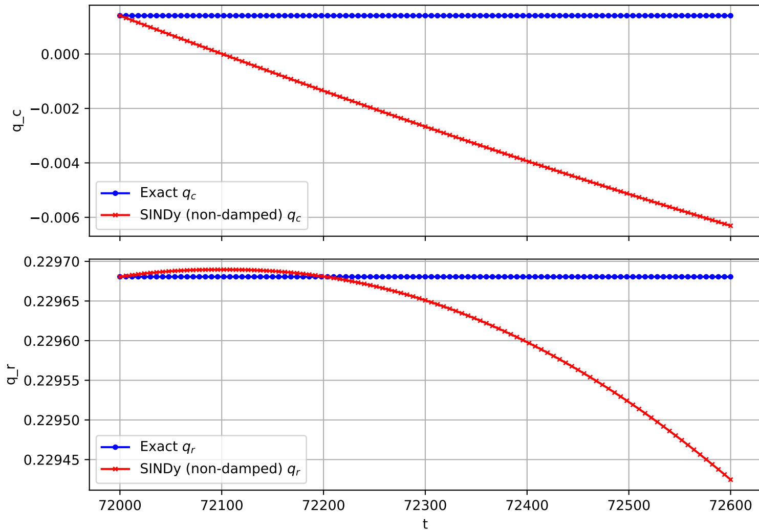
Trajectory 2365 (non-damped)
