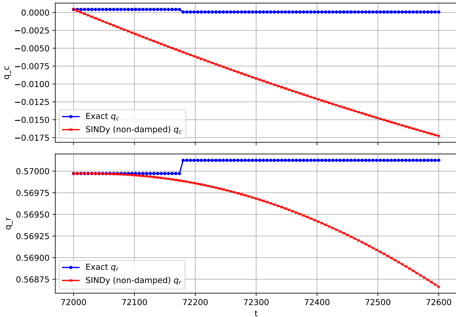
Trajectory 2379 (non-damped)
