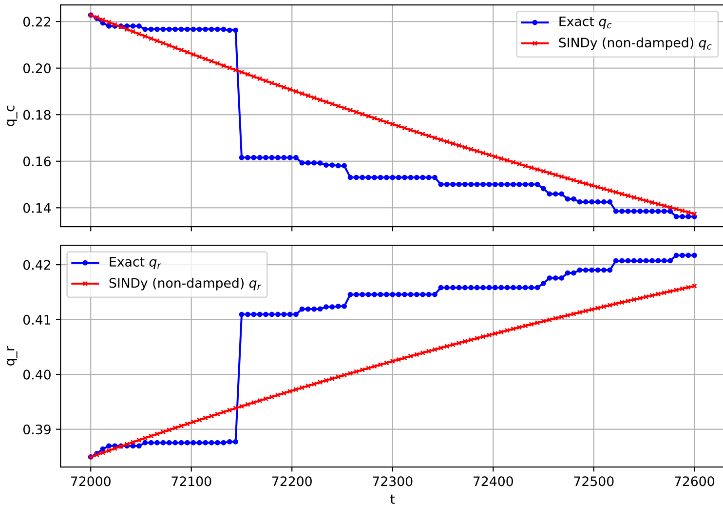
Trajectory 2382 (non-damped)
