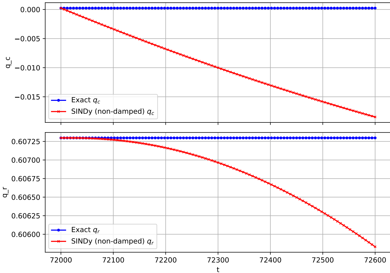
Trajectory 2385 (non-damped)
