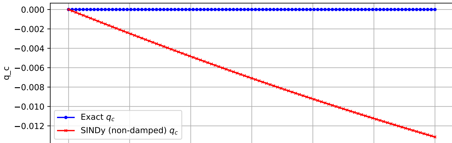
Trajectory 2388 (non-damped)
