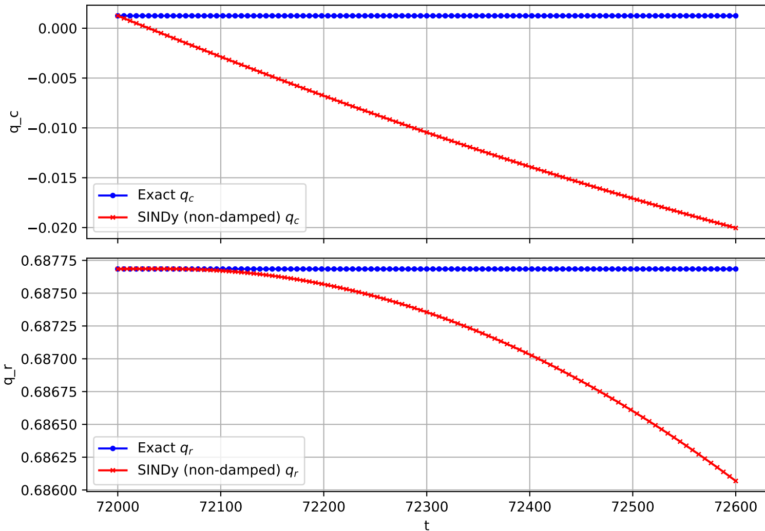
Trajectory 2393 (non-damped)
