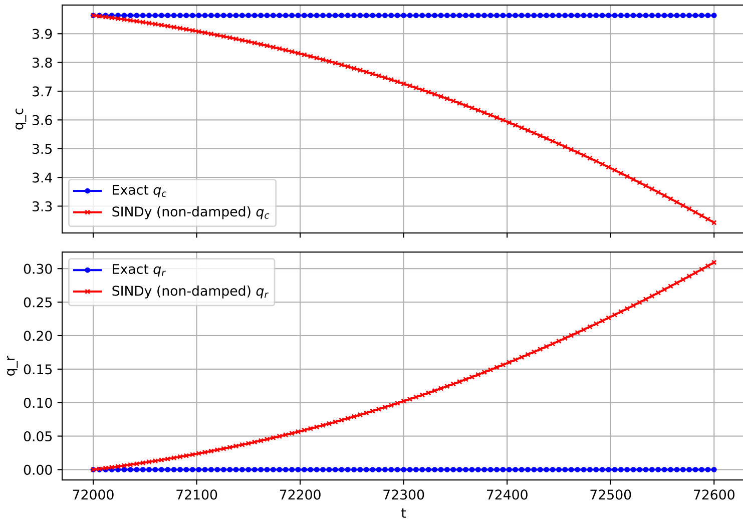
Trajectory 24 (non-damped)
