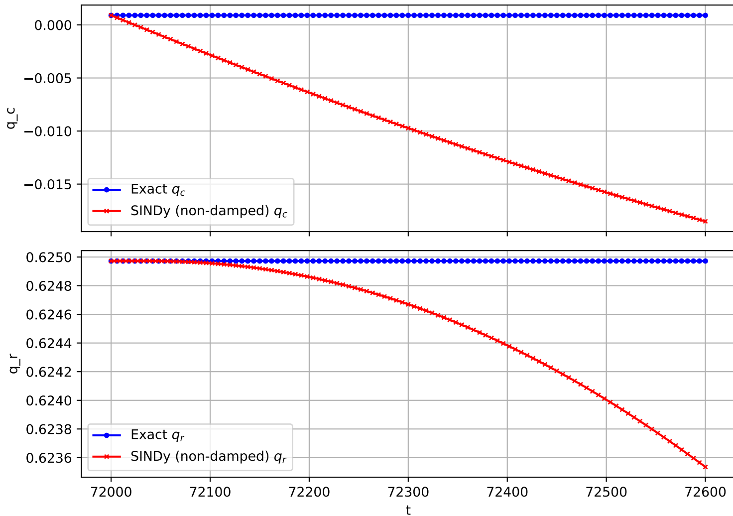
Trajectory 2406 (non-damped)
