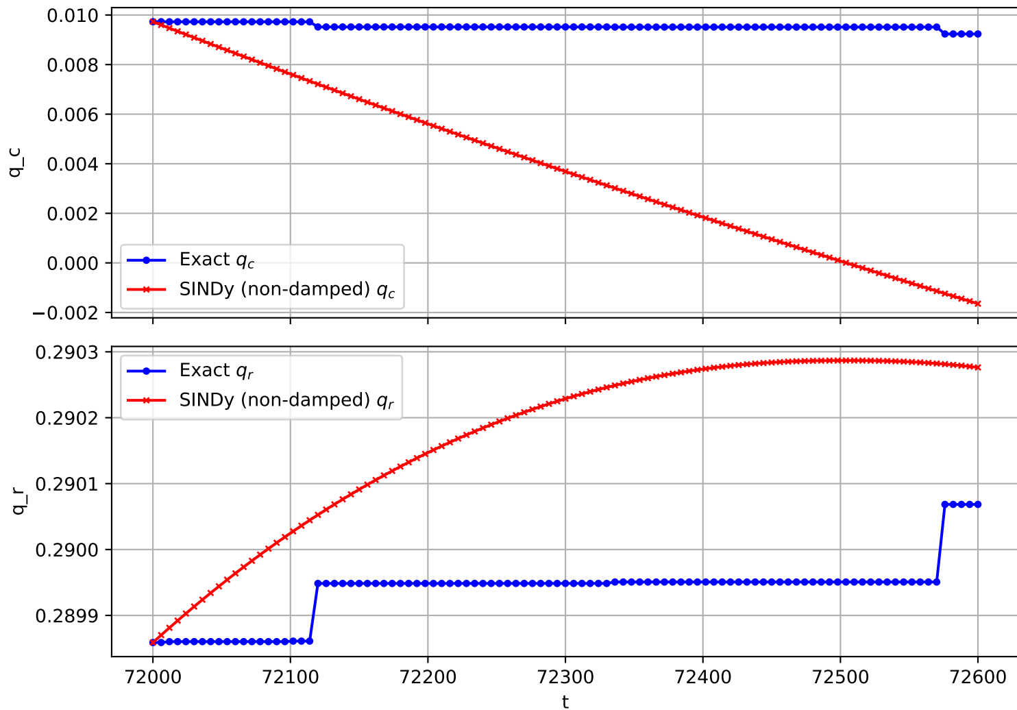
Trajectory 2410 (non-damped)
