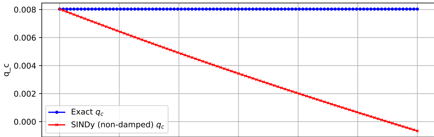
Trajectory 2418 (non-damped)
